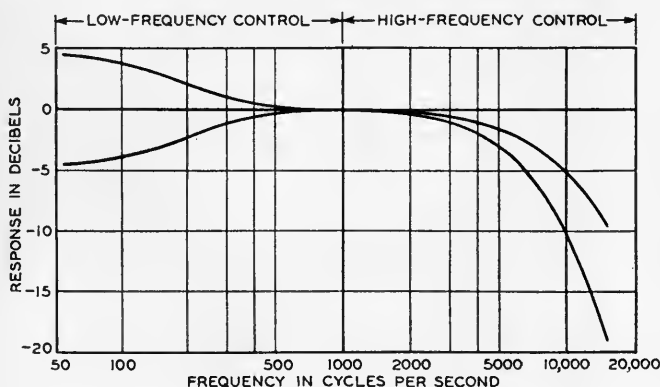
FIG. 5. Frequency characteristics of the stereophonic system obtainable by manipulating the six keys that are located on the top of the enhancement control unit.
